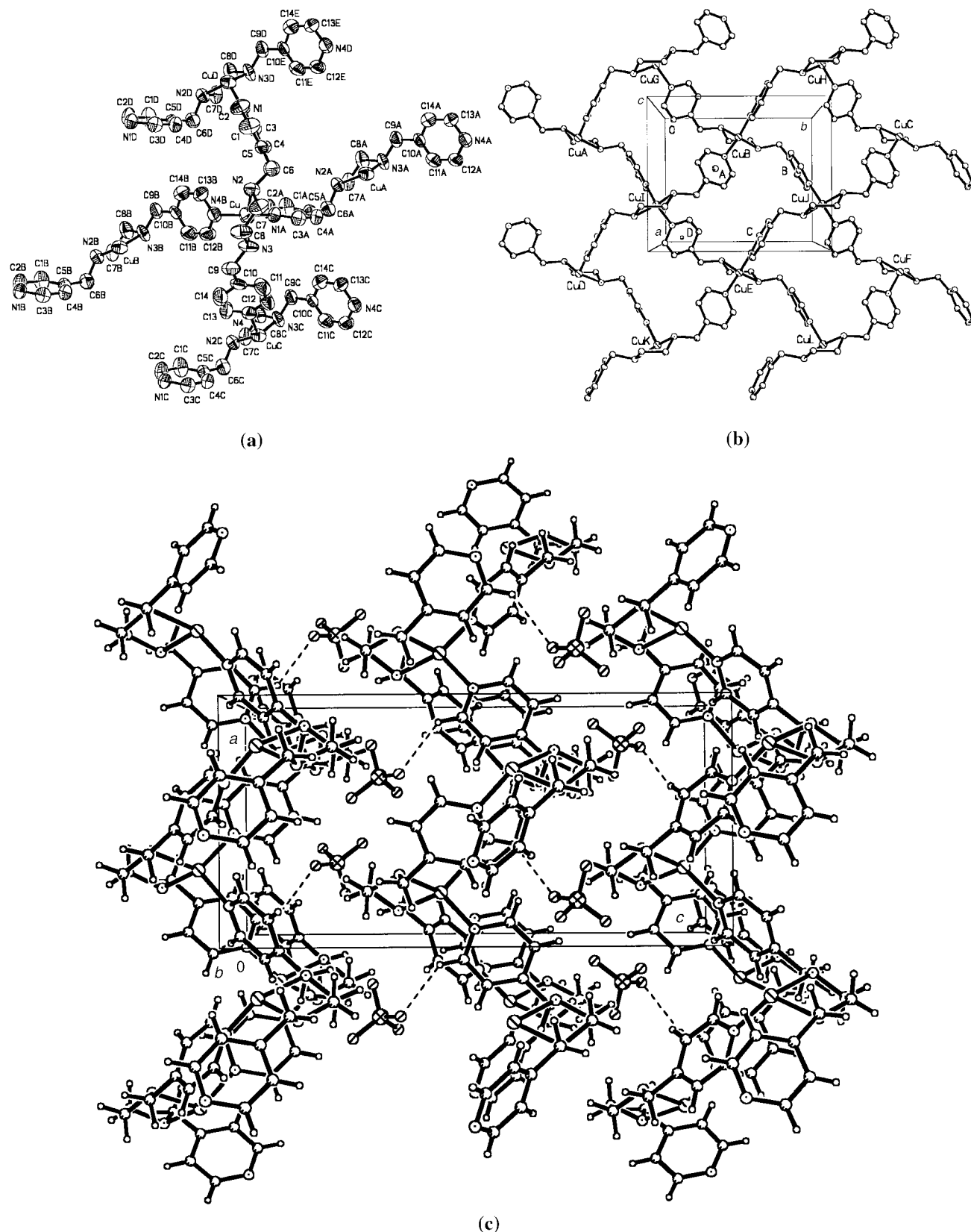
Fig. 3 (a) Crystal structure of the cationic moiety of [\text{Cu}(\text{BPDH})]\text{ClO}_4 3. (b) Infinite grid structure of 3. (c) Crystal packing diagram of 3 with hydrogen bonds indicated by dashed lines.
